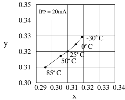
Ambient Temperature vs. Chromaticity Coordinate ( λ D)
